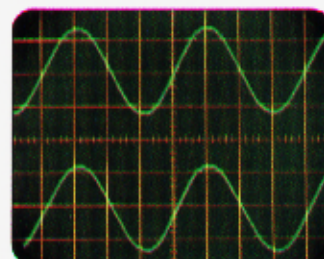
Input and output waveforms power factor:1.0 Load:100% (5msec/cm)
