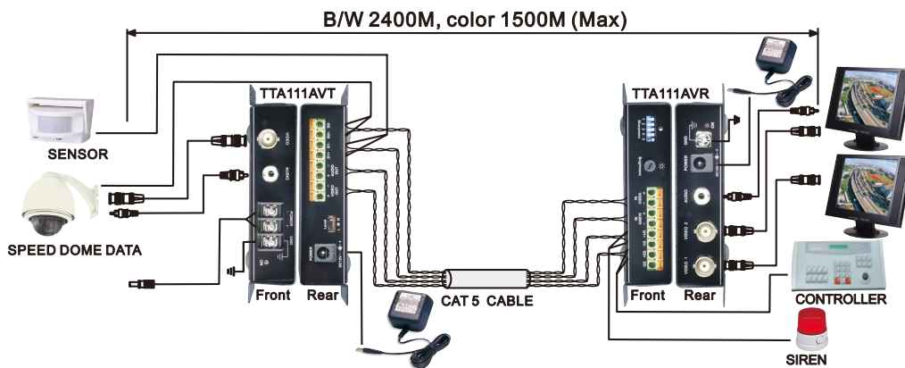
TTA111AVT Transmitter
