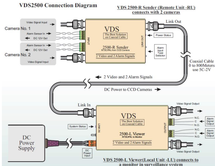
VDS2500 Connection Diagram
